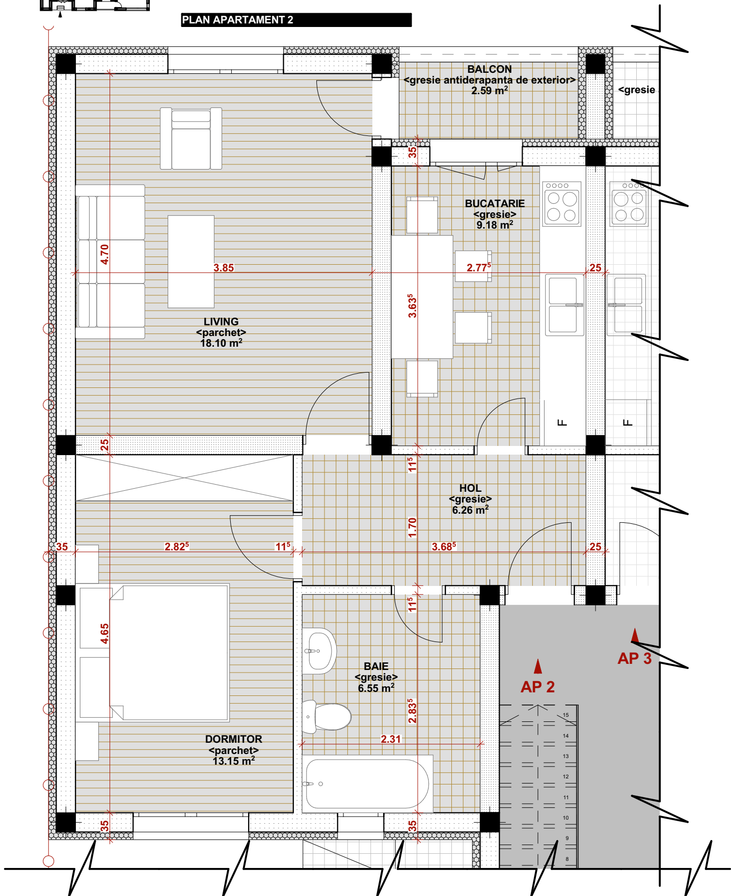
PLAN PARTER. APARTAMENT 2 - Suprafata utila 53.24 mp, Suprafata balcon 2.59 mp
