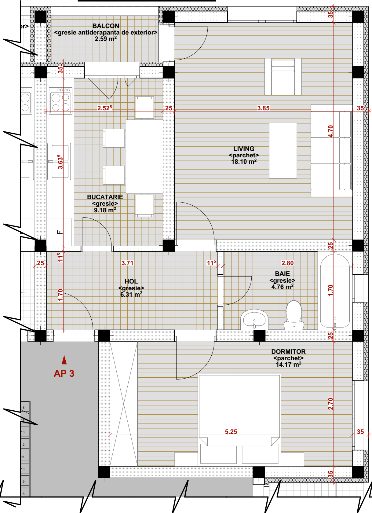
PLAN PARTER .APARTAMENT 3 - Suprafata utila 52.52 mp, Suprafata balcon 2.59 mp
